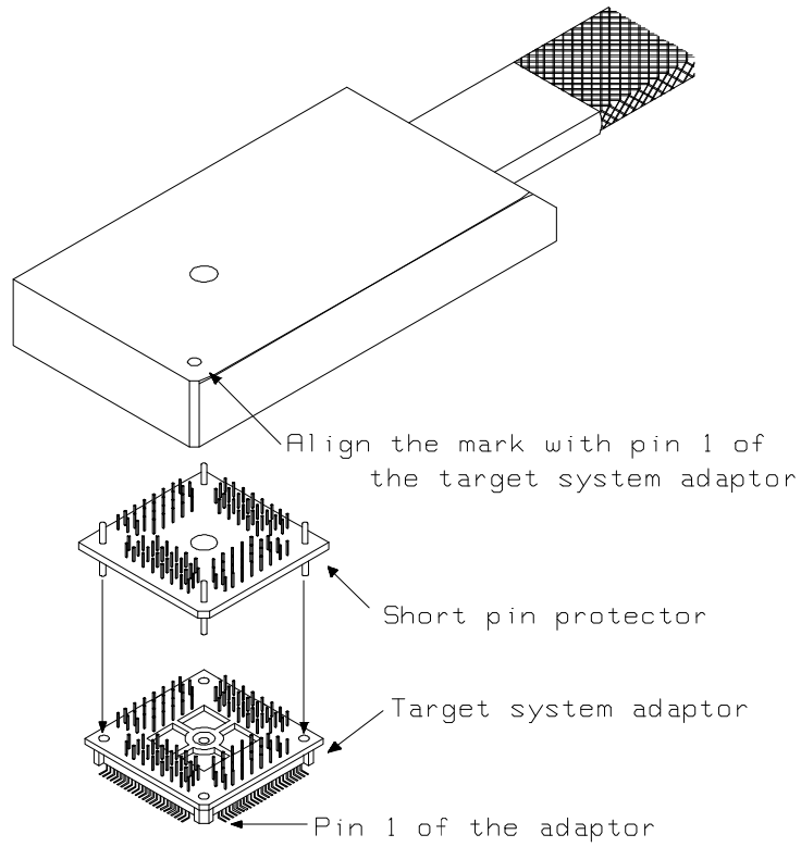
Figure 3-1. Installing the Target System Probe
