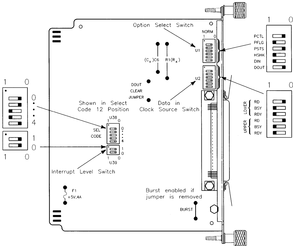
Figure 5-6. HP 98622A GPIO Switches and Jumpers
