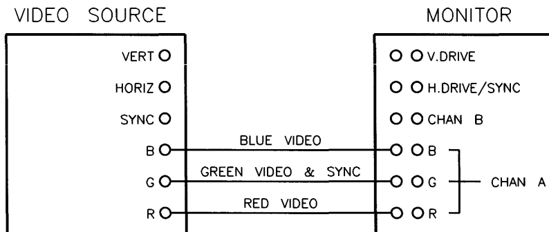
Figure 8-5. HP 13279B Cable Connections.
