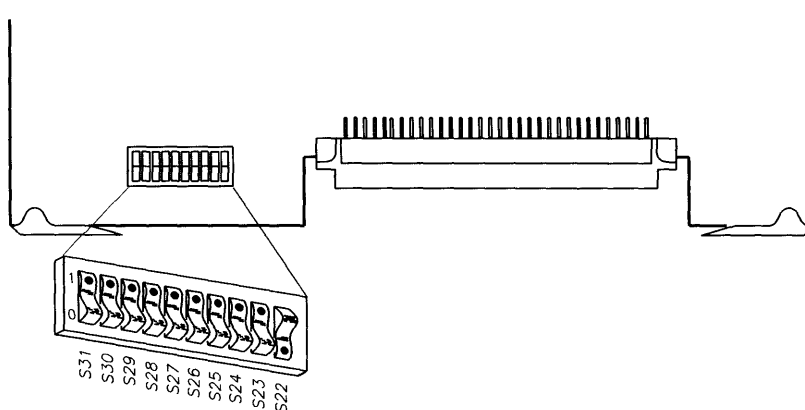
Figure 3-1. Setting switches on the new HP 98258A RAM board
