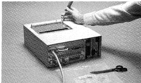
Figure 2-13. Installing the Flat-head Screw
