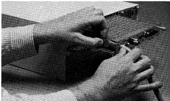
Figure 5-53. Cable Clamp
