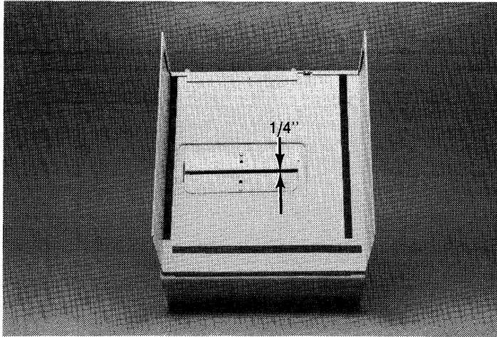
Figure 2-3. Sliding Clips
