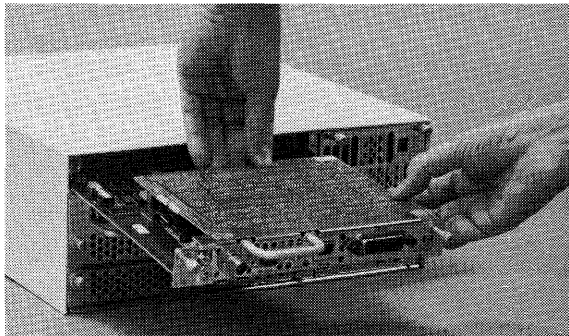
Figure 5-49. Joining the Connectors
