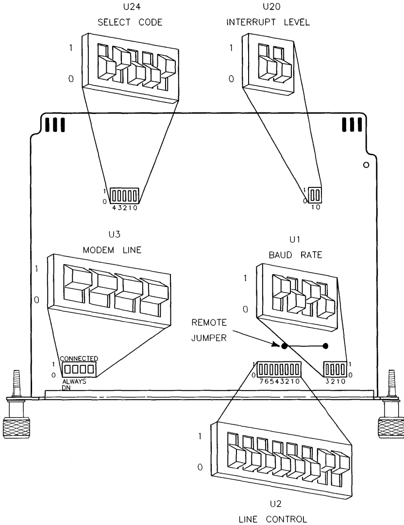
Figure 5-14. HP 98626A RS-232C Serial Interface Switches
