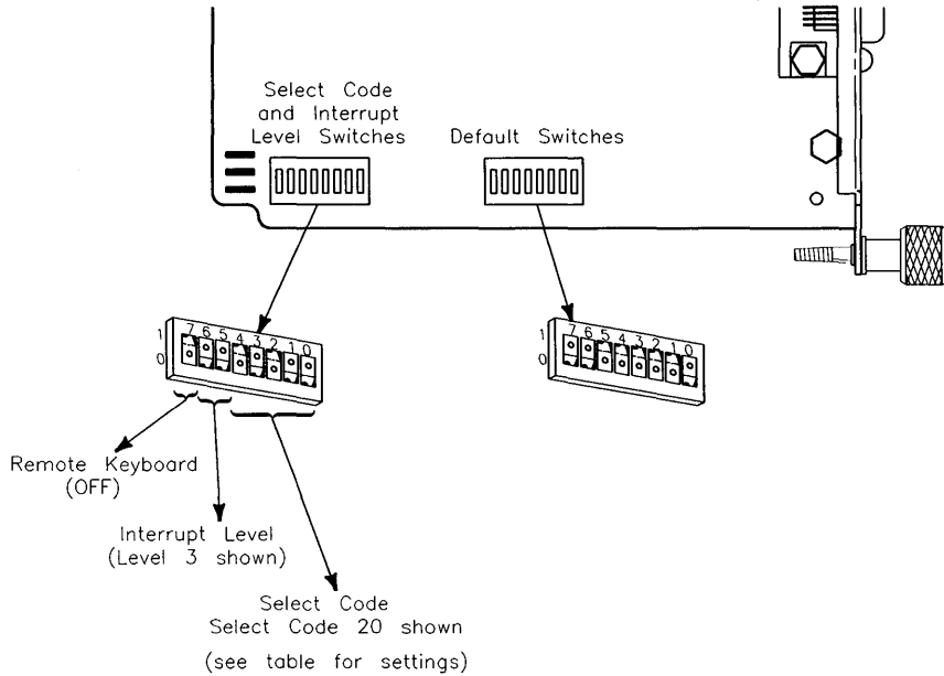
Figure 5-24. 98628A Datacomm Interface Switches
