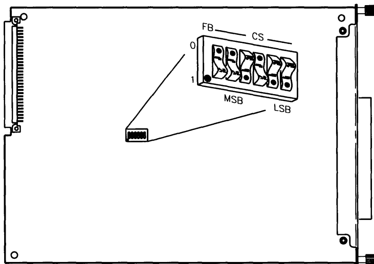
Figure 5-41. HP 98725A LGB Interface Switches
