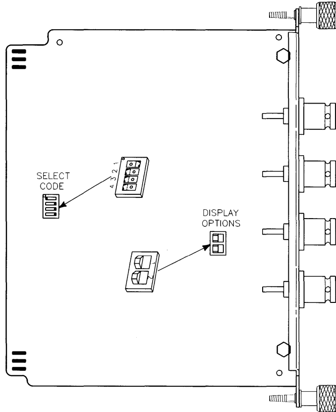
Figure 5-23. HP 98627A Color Video Output Interface Switches
