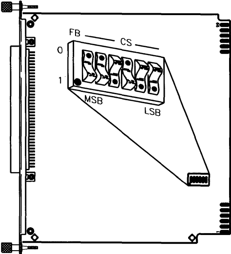
Figure 5-40. HP 98724A LGB Interface Switches
